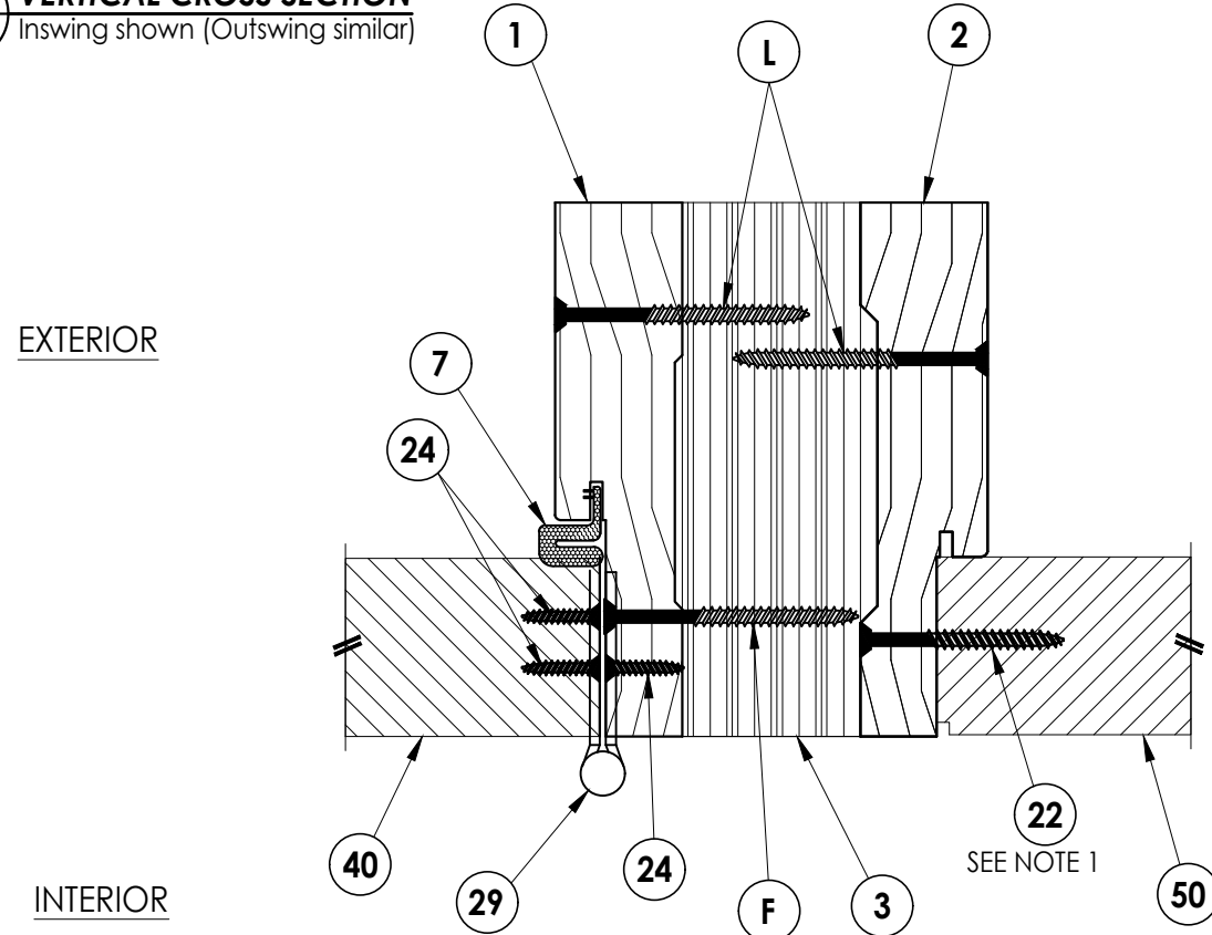
4 HORIZONTAL CROSS SECTION 8 Inswing shown (Outswing similar)
