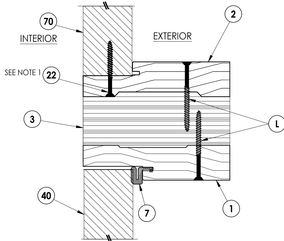
2 VERTICAL CROSS SECTION 8 Inswing shown (Outswing similar)
