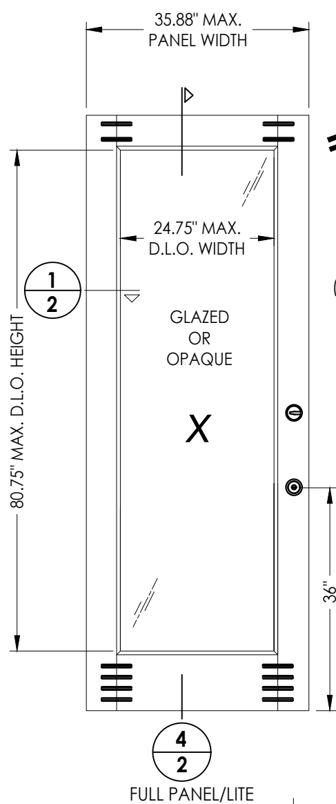
40 WOOD DOOR PANEL Glazed or Opaque
