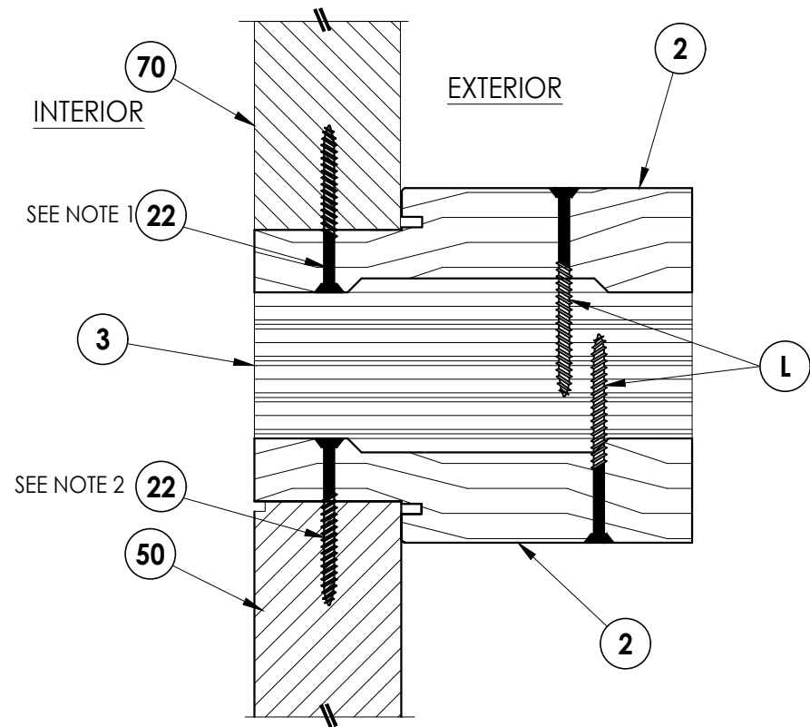
1 VERTICAL CROSS SECTION 8 Inswing shown (Outswing similar)
