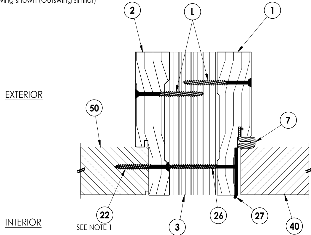
3 HORIZONTAL CROSS SECTION 8 Inswing shown (Outswing similar)
